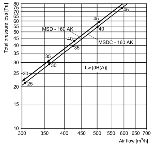
Figure 4: Pressure loss and sound power level MSD 160 – AK and MSDC 160 – AK
