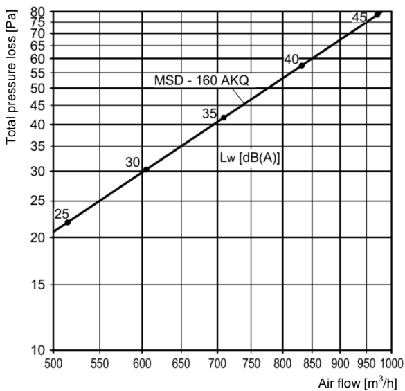
Figure 5: Pressure loss and sound power level MSD 160 – AKQ
