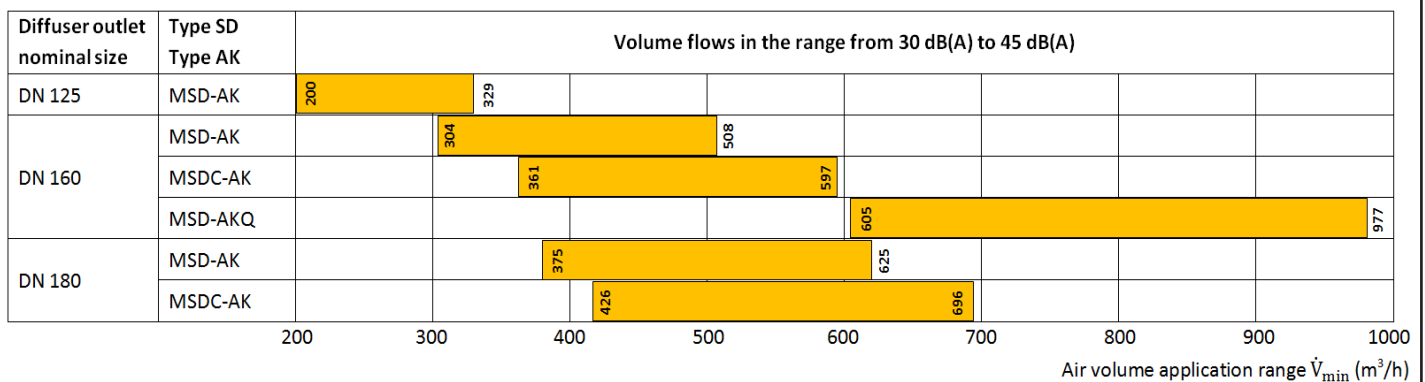
Figure 2: Recommended air volume application ranges for multi swirl diffusers type MSD and MSDC with plenum box type AK or AKQ
