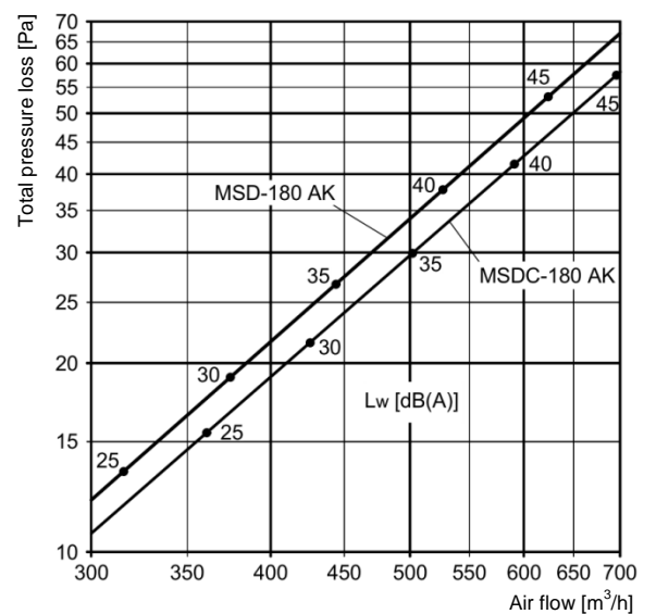
Figure 6: Pressure loss and sound power level MSD 180 – AK and MSDC 180 – AK
