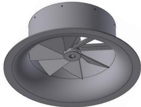
Type SDC swirl diffuser with curved blades
