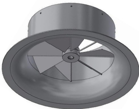
Type SD swirl diffuser with flat blades
