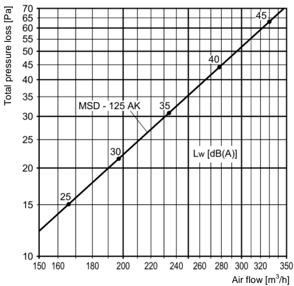
Figure 3: Pressure loss and sound power level MSD 125 – AK
