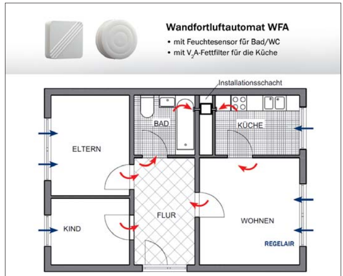
Abb. 4: Wandfortluftautomat WFA
